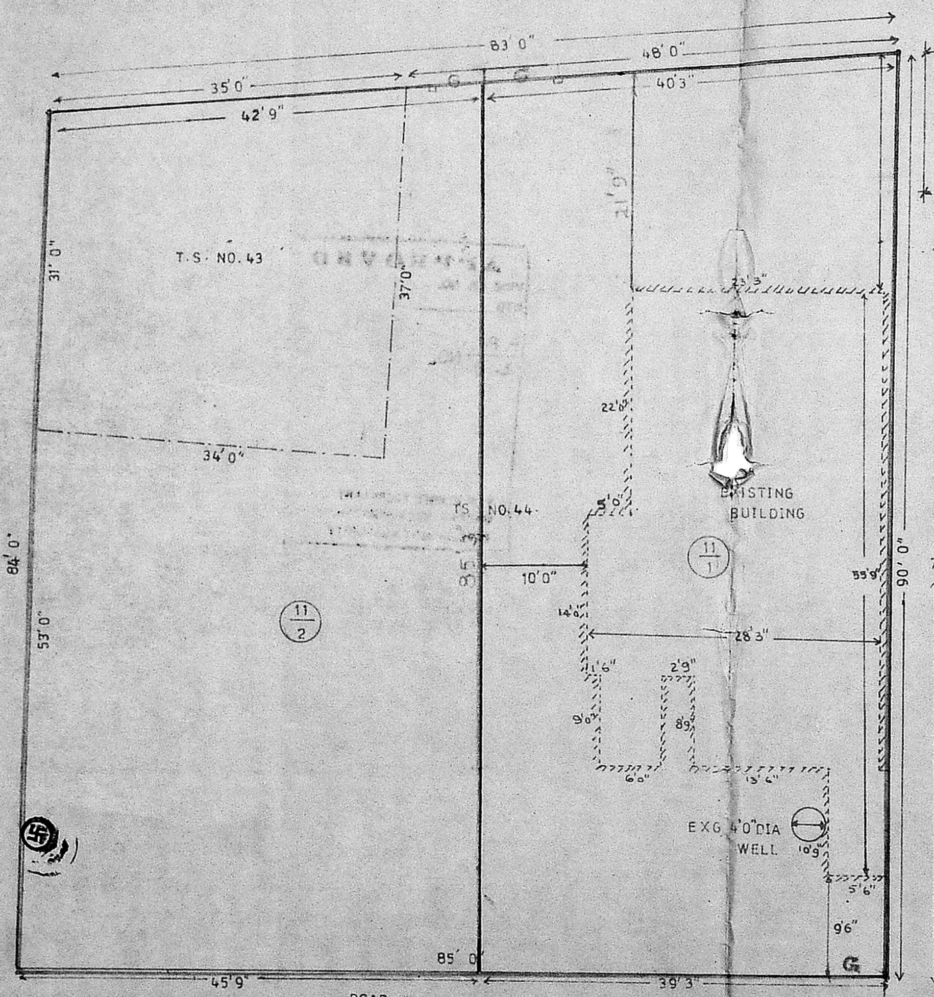
PLAN Scale 1" = 10'
